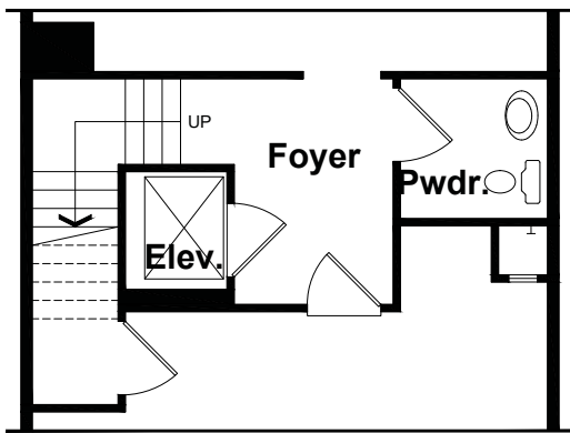
Optional Elevator Entry Level
